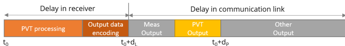
Figure 2-3: PVT latency.
